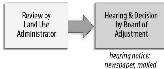
Figure 14-4: Variance Process
